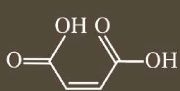
Maleic acid
