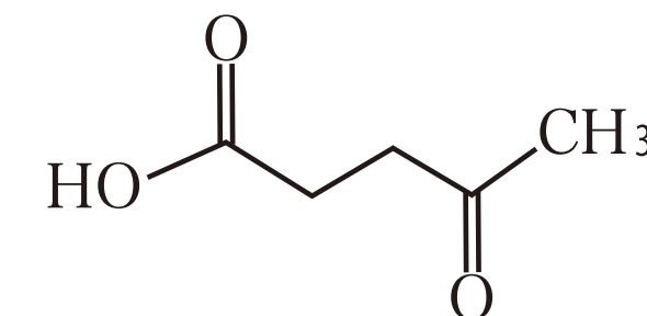
Levulinic acid
