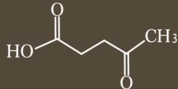
Levulinic acid
