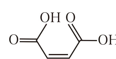
Maleic acid
